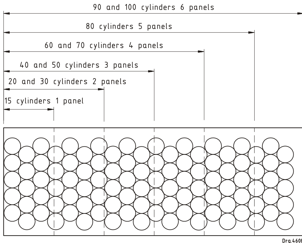
b) Diagram illustrating number of panels to bank size
