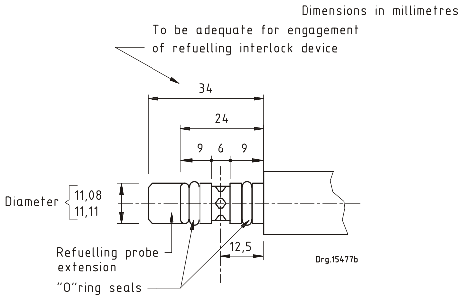
Male probe (the fitting on the refuelling hose)
