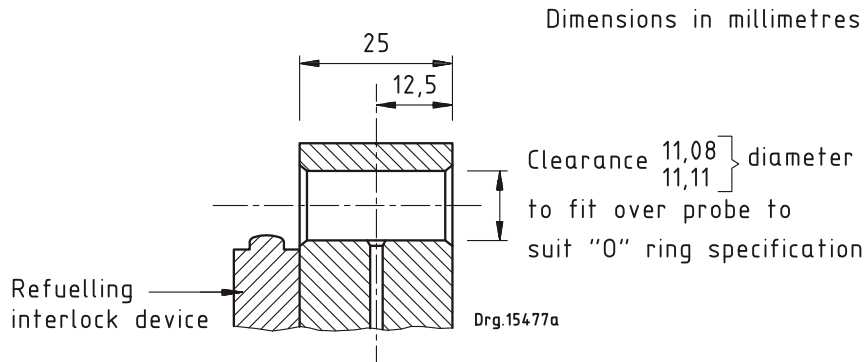
Female (the fitting on the vehicle)
