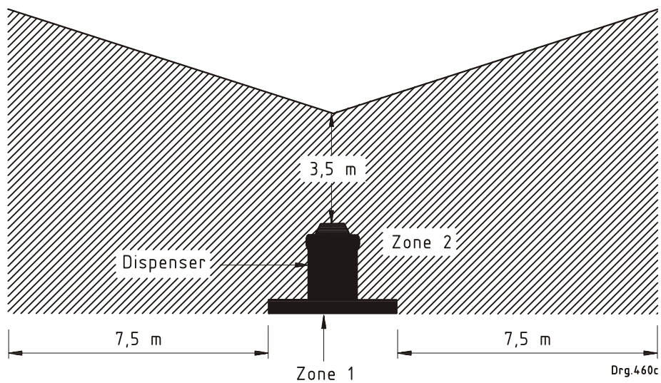
a) Front view of the canopy
