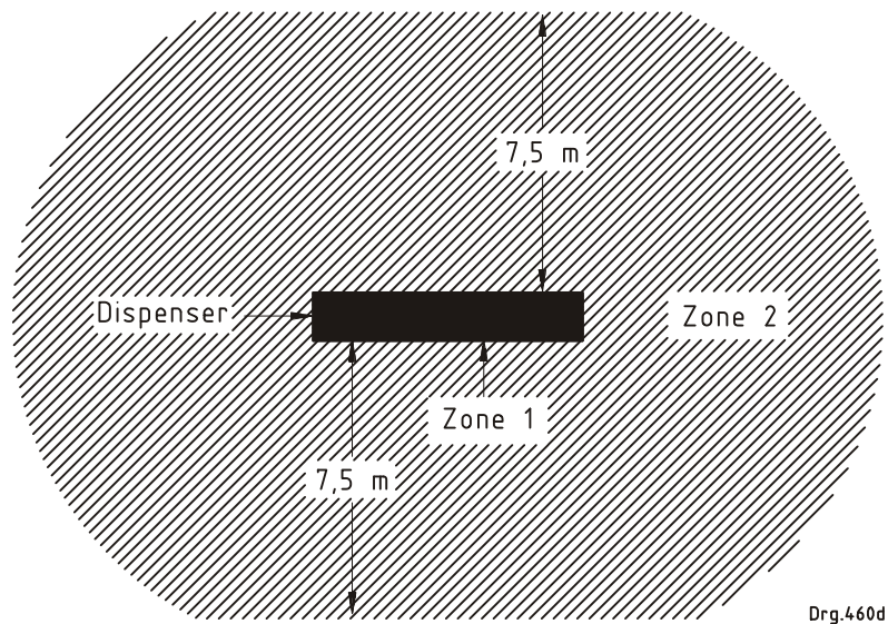
b) Top view of the canopy
